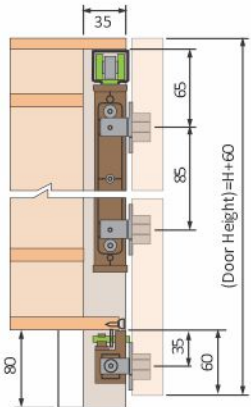
Technical Detail for AVSLD-403 & AVSLD-404
